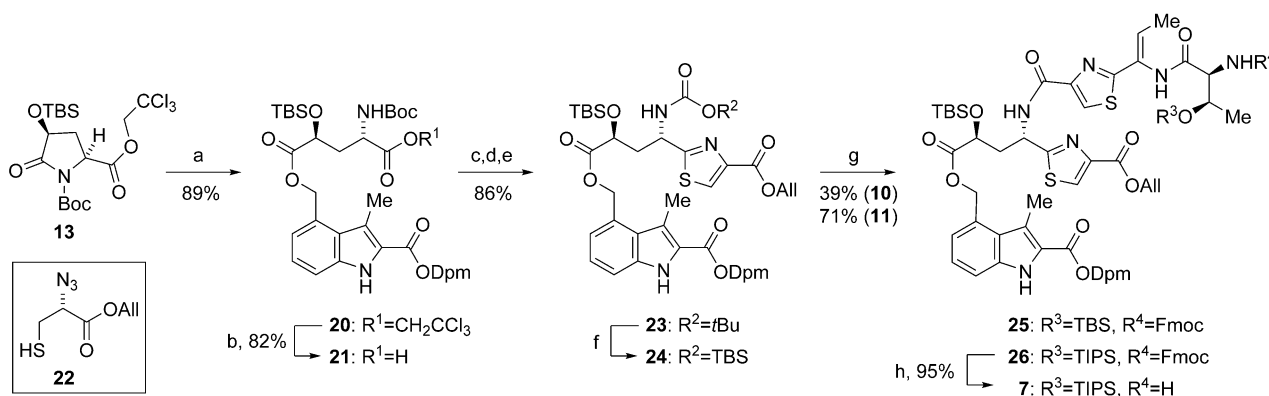
Scheme 2. Synthesis of the indole-thiazole building block. Reagents and conditions: a) 12 (0.5 equiv), NaH (1.25 equiv), THF, −78 °C, 2 h (98% b.r.s.m.); b) Zn (36 equiv), 1 M KH 2 PO 4 , THF, 45 °C, ultrasound, 10 h (95% b.r.s.m.); c) 22 (1.5 equiv), PyAOP (1.2 equiv), EtN i Pr 2 (2.5 equiv), 0 °C → 20 °C, 3 h; d) PPh 3 (1.5 equiv), THF, −20 °C → 20 °C, 2 h; then 40 °C, 14 h; e) DBU (2.1 equiv), BrCCl 3 (1.05 equiv), CH 2 Cl 2 , −20 °C, 1 h; f) TBSOTf (11 equiv), 2,6-lutidine (22 equiv), CH 2 Cl 2 , 0 °C → 20 °C; g) 10 or 11 (1 equiv), HATU (1.4 equiv), HOAt (6.5 equiv), NaHCO 3 (3 equiv), THF, 0 °C → 20 °C, 48 h; h) DBU (5% in CH 2 Cl 2 ), −20 °C, 5 min. b.r.s.m. = based on recovered starting material.
