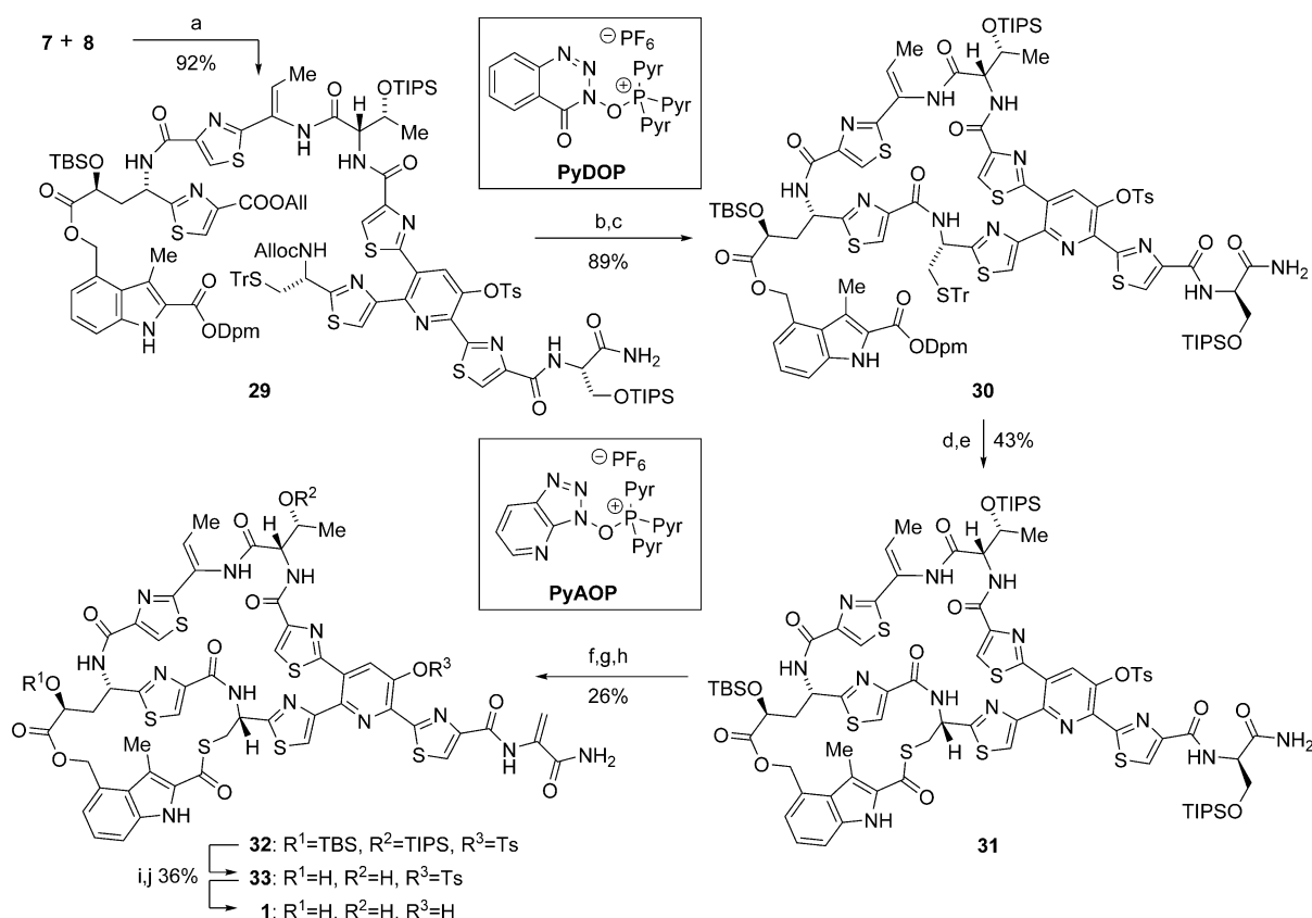
Scheme 4. Completion of the synthesis. Reagents and conditions: a) PyDOP (2 equiv), EtNiPr 2 (2.2 equiv), THF, 0°C, 15 min, 20°C, 2 h; b) [Pd(PPh 3 ) 4 ] (20 mol%), PhSiH 3 (20 equiv), THF, 0°C, 30 min; c) HATU (5 equiv), EtNiPr 2 (30 equiv), THF, 0°C, 15 min; d) anisole/TFA/Et 3 SiH (8:5:4), -20°C, 30 min; then 0°C, 4 h; e) PyAOP (1.2 equiv), EtNiPr 2 (2.3 equiv), THF, 0°C, 15 min, then 20°C, 15 h; f) CH 3 CN/conc. HF (24:1), 0°C, 25 h, 75% (90% b.r.s.m.); g) methanesulfonyl chloride (100 equiv), 2,6-lutidine/CH 2 Cl 2 (1:10), 0°C→20°C, 0.5 h; h) DBU (2% in CH 2 Cl 2 ), -78°C→-35°C, 4.5 h (35%, two steps); i) Et 3 N×3HF/THF (1:9), 0°C→20°C, 27 h; j) HOBT (10 equiv), EtNiPr 2 (7 equiv), DMF, 0°C→20°C, 1.5 h. Pyr = pyrrolidine-1-yl.
