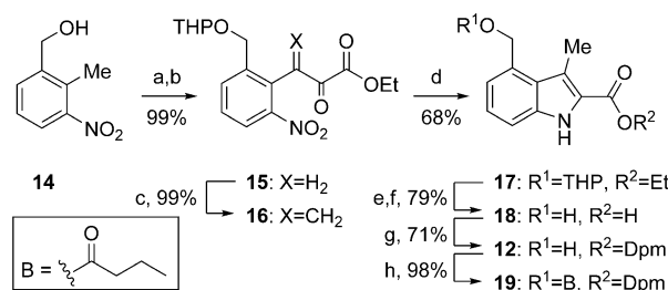
Scheme 1. Synthesis of indole 12 . Reagents and conditions: a) Dihydropyran (2 equiv), PPTS (0.1 equiv), 1,2-dichloroethane, 20 °C, 18 h; b) NaH (3 equiv), diethyl oxalate (6 equiv), DMF, 0 °C → 20 °C, 18 h; c) dimethylmethyleneiminium chloride (3 equiv), NEt 3 (3 equiv), 20 °C, 13 h; d) cat. 10 % Pd/C (10 wt %), 1–4 bar H 2 , 4 Å molecular sieves (20 wt %), THF/ i PrOH (1:1), 18 h; e) aq. NaOH (2.5 M, 3 equiv), EtOH, reflux, 30 min; f) AcOH (70 %), 20 °C, 18 h; g) diphenyldiazomethane, cat. TFA, THF, 60 °C, 3 h; h) butyric anhydride (2 equiv), Et 3 NiPr 2 (4 equiv), DMAP (0.1 equiv), THF, 0 °C → 20 °C, 13 h.
