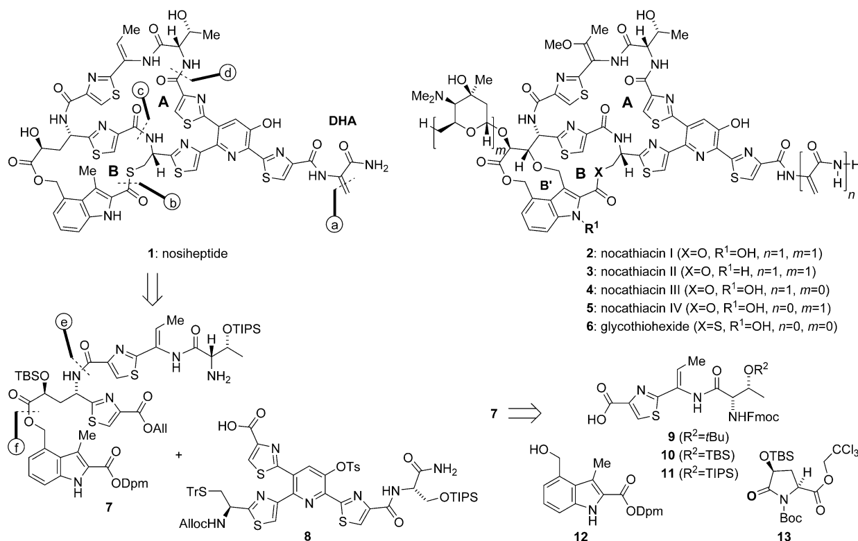
Figure 1. Chemical structures of class e thiopeptide natural products and retrosynthetic disconnection of nosiheptide. All = Allyl, Alloc = Allyloxycarbonyl, Boc = tert -Butyloxycarbonyl, DBU = 1,8-Diazabicyclo[5.4.0]undec-7-en, DMAP = Dimethylaminopyridine, Dpm = Diphenylmethyl, Fmoc = Fluorenylmethyloxycarbonyl, HATU = O-(7'-Azabenzotriazol-1'-yl)-1,1,3,3-tetramethyluronium hexafluorophosphate, HOAt = 1-Hydroxy-7-azabenzotriazole, PPTS = Pyridinium 4-methylphenylsulfonate, PyAOP = (7-Azabenzotriazol-1-yloxy)tripyrrolidinophosphonium hexafluorophosphate, PyDOP = (3,4-Dihydro-4-oxo-1,2,3-benzotriazin-3-yl)oxytripyrrolidinophosphonium hexafluorophosphate, TBS = tert -Butyldimethylsilyl, TIPS = Triisopropylsilyl, Tr = Triphenylmethyl, Ts = 4-Methylphenylsulfonyl.
