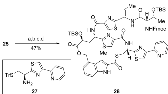
Scheme 3. Completion of the fully equipped B-ring model. Reagents and conditions: a) [Pd(PPh 3 ) 4 ] (20 mol %), PhSiH 3 (8.6 equiv), THF, 0 °C, 20 min, 93 %; b) PyBOP (2.1 equiv), Et 3 N (2.5 equiv), 27 (1.5 equiv), DMF, 0 °C → 20 °C, 16 h, 77 %; c) anisole/TFA/Et 3 SiH (8:5:4), -25 °C → 0 °C, 24 h; d) PyAOP (1.2 equiv), Et 3 N (2.2 equiv), THF, 0 °C, 15 min, 20 °C, 1 h, 66 %.
